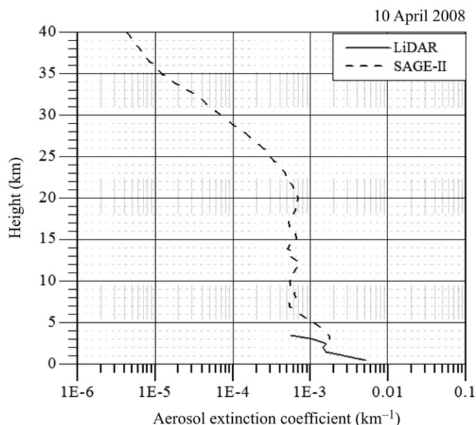
Fig. 4. Height profile of aerosol extinction coefficient retrieved from SAGE II and LIDAR.
